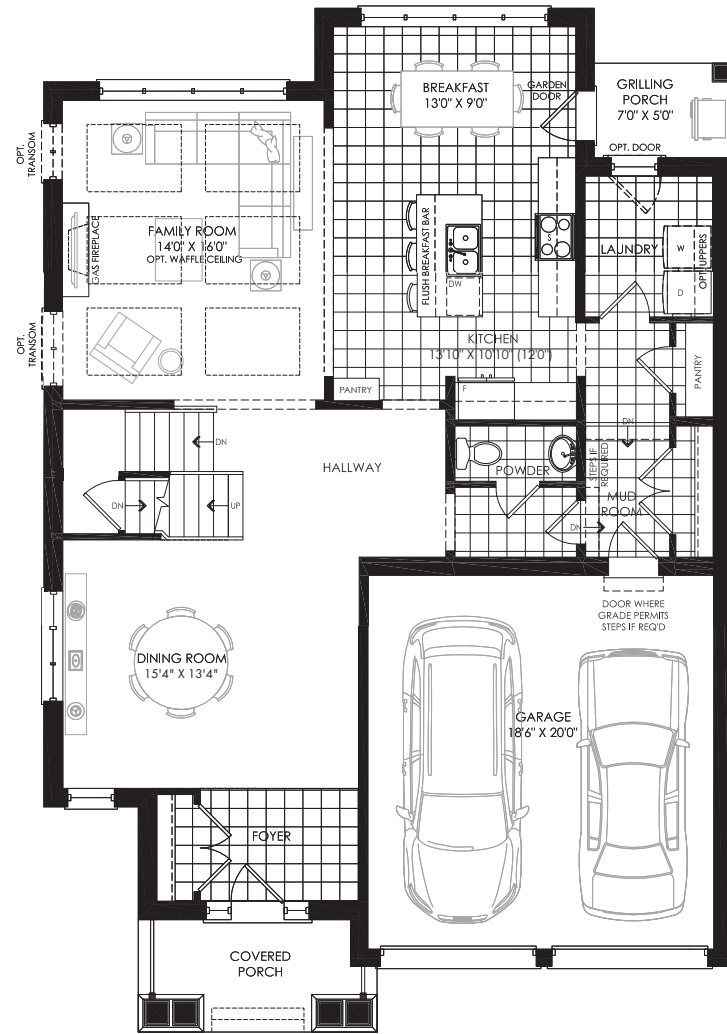
GROUND FLOOR PLAN ELEV. 'A'
