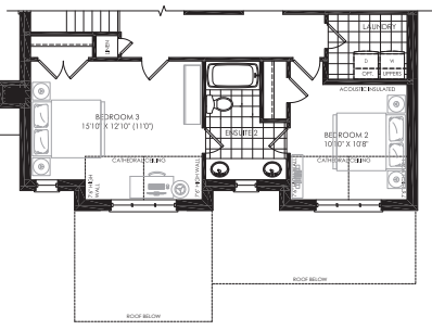
PARTIAL SECOND FLOOR FLEX PLAN ELEV. 'D' W/ LAUNDRY
