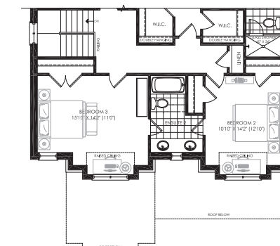
PARTIAL SECOND FLOOR PLAN ELEV. 'B'
