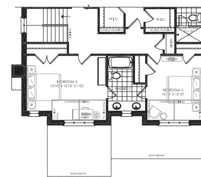
PARTIAL SECOND FLOOR PLAN ELEV. 'D'
