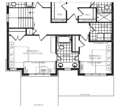
PARTIAL SECOND FLOOR FLEX PLAN ELEV. 'A' W/ LAUNDRY
