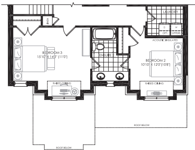
PARTIAL SECOND FLOOR FLEX PLAN ELEV. 'B' W/ LAUNDRY
