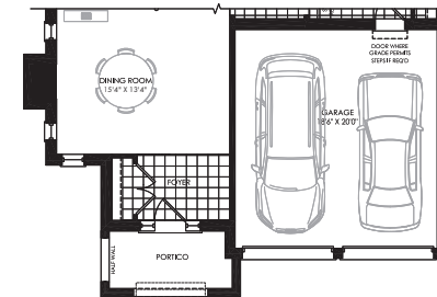
PARTIAL GROUND FLOOR PLAN ELEV. 'D'
