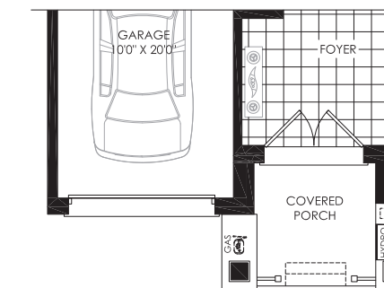
PARTIAL GROUND FLOOR PLAN ELEV. BB
