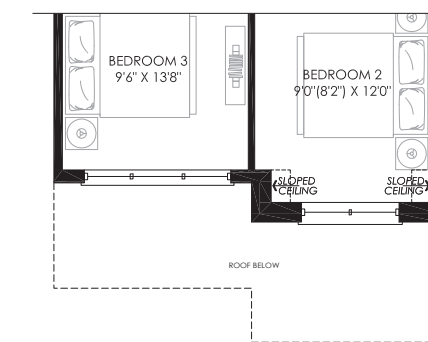
PARTIAL SECOND FLOOR PLAN ELEV. BB
