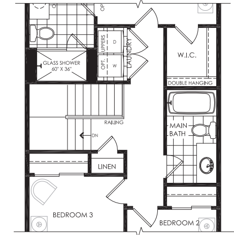
PARTIAL SECOND FLOOR FLEX PLAN W/ LAUNDRY ELEV. AC & BB
