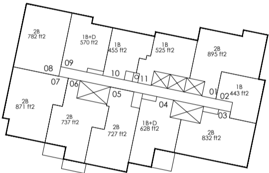
11th Floor
