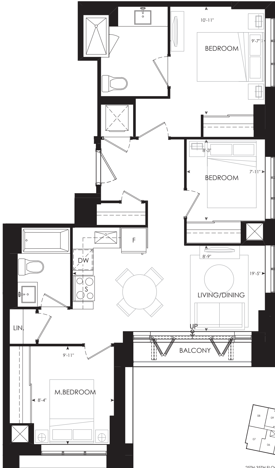
25TH-35TH FLOORPLAN
